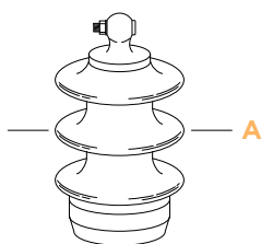
Example of a typical cross section of an HVCE with the dimensions representing that of the insulator profile
