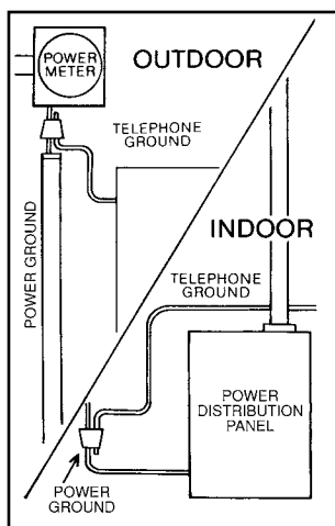
Consumer Entrance Service
